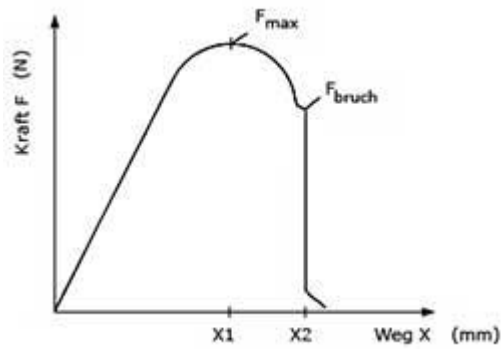
Force-Pad-Diagram van universele controlemachine ZPM
